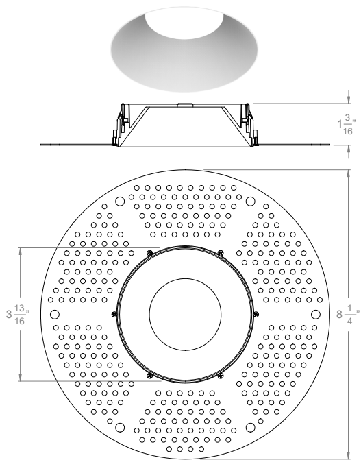
A3-1R 3" Acrobat Round Trimless Mud Plate
