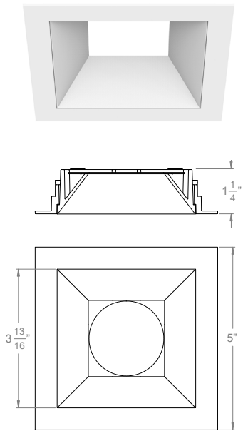
A3-1S 3" Acrobat Square Standard Trim
