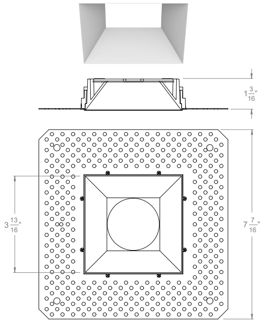
A3-1S 3" Acrobat Square Trimless Mud Plate
