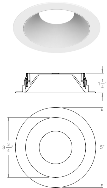
A3-1R 3" Acrobat Round Standard Trim
